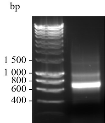
Figure 2. Sample of amplified VHH1 of approximately 700 bp visualised on a 1% agarose gel
