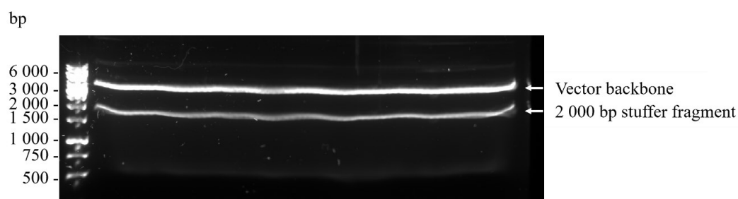
Figure 4. Preparative 0.7% agarose gel containing 1× SYBR TM safe DNA gel stain of the vector backbone (upper band) and stuffer fragment (lower band) after SfiI digestion of pADL23c phagemid vector prior to gel extraction. The sizes in base pairs of a DNA ladder run in parallel are shown.
