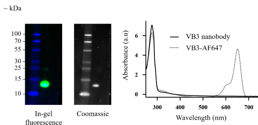
Figure 10. Conjugation of Alexa Fluor™ 647 to VB3 nanobody (VB3-AF647) expressed in pOPINVHH_Cys as determined by in-gel fluorescence (left), InstantBlue® staining (middle), and absorbance profile (right)
