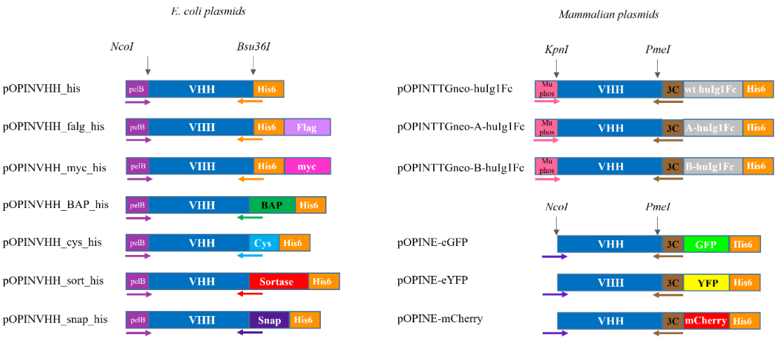
Figure 8. Details of the primers, restriction enzymes, and tags present in each of the vectors in the bacterial and mammalian toolboxes. Abbreviations used: VHH, nanobody; BAP, biotin acceptor peptide/Avi-Tag™; wt, wild-type; huIg1Fc, human Ig1 Fc.
