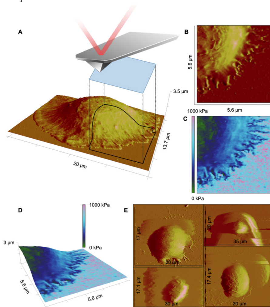
Figure 2. AFM-based elasticity mapping (PeakForce QNM) and data analysis.
