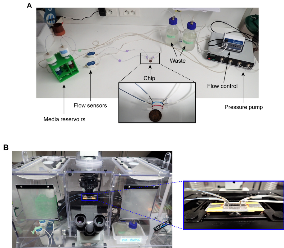
Figure 4. Microfluidic device setup. A. Media reservoirs are pressurized with Fluigent MFCS pressure pump resulting in flow through the flow sensors, into the chip and then to waste. Flow sensors and pressure pump are connected to the flow-rate control module, which maintains a constant flow through the system. Nutrient supply and media conditions can be changed in real time. B. Microfluidic chip mounted on a microscope. This figure is modified from the original article (Marinkovic et al. , 2019).
