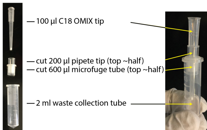
Figure 2. Centrifugal device for solid phase extraction of tryptic peptides for LC-MS/MS.
