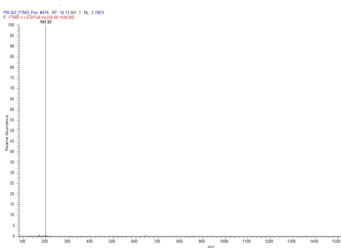
Figure 3. Mass spectrum of 2-Hydroxyphenazine, m/z [M + H]^+ 197.07.
