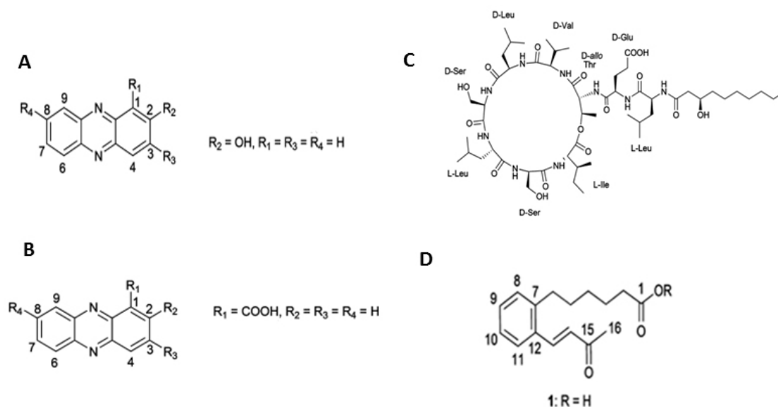
Figure 1. Structures of the compounds isolated from Pseudomonas aurantiaca and Pseudomonas chlororaphis .
