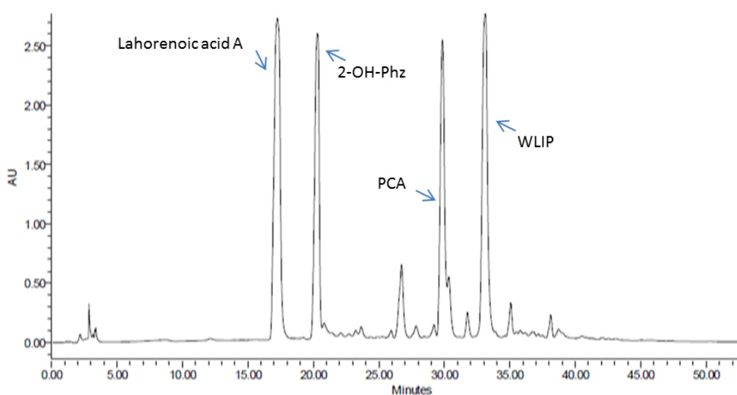
Figure 5. HPLC analysis of enriched P. aurantiaca PB-St2 fractions of detected metabolites.
