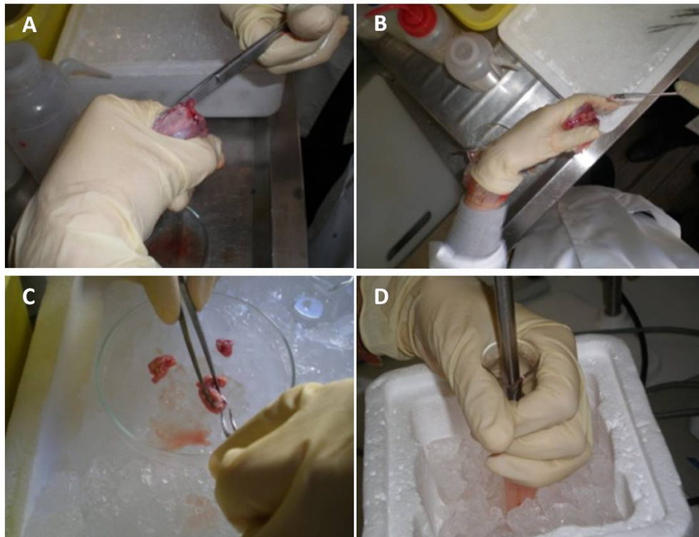
Figure 2. Illustrative images of brain dissection and homogenization. Cut the cranium carefully from the neck to the nose through the lateral cranial sutures (A). Remove the intact brain from the cranial box using a small spatula (B). Then, remove the cerebellum, olfactory bulbs and white matter using fine dissection forceps and keep the brain cortices (C). Finally, homogenize brain tissue, at 4 °C, in 10 ml PBS using a Potter-Elvehjem with PTFE pestle and glass tube, at 800 rpm/min (D).
