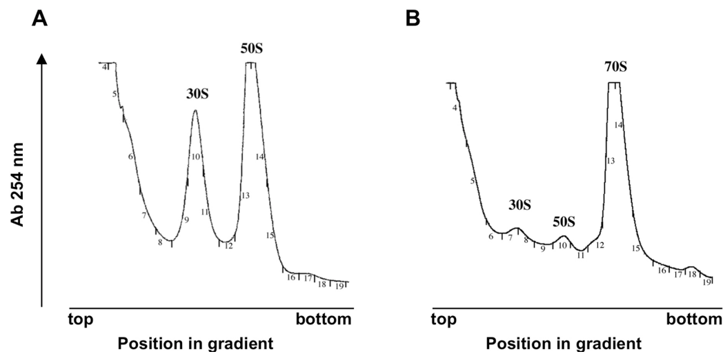
Figure 2. Sedimentation profiles showing the free subunits and 70S vacant ribosomes. The Synechocystis S30 supernatant was fractionated on a 10-30% sucrose density gradient in the presence of 1 mM (A) or 10 mM (B) Mg^{2+} . Small numbers refer to collected fractions. Adapted from (Galmozzi et al. , 2016).
