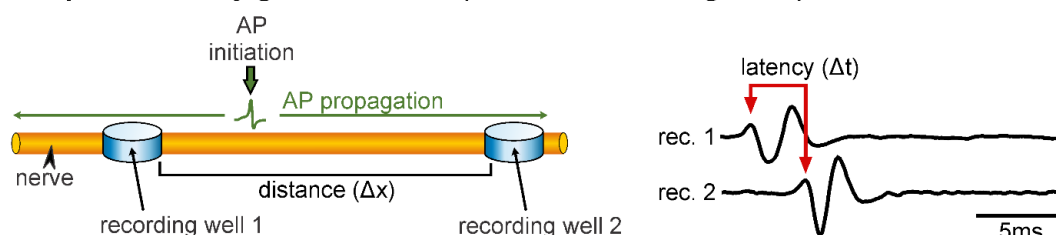
Figure 1. Representation of the electrode placement for measuring conduction velocity of stimulated APs (A) and spontaneously generated APs (B & C). A. Left: APs are initiated within the stimulation well and propagate along the axon (green arrows) towards the recording well. Note that APs propagate bi-directionally but are only detected at the recording site. \Delta x represents the distance between the stimulation and recording wells. Right: Extracellular recording of a nerve showing the latency ( \Delta t ) between the onset of the stimulation (stim. artifact) and the AP (gray box). B. Left: Correct electrode placement for measuring conduction velocity of spontaneously generated APs. Recording wells need to be placed in such a way that the AP is passing the wells without being initiated in-between the wells. Right: The latency in AP occurrence at the two recording sites reflects the time the AP needs to propagate from recording 1 to recording 2. C. Left: Incorrect electrode placement for measuring conduction velocity of spontaneously generated APs. Right: The latency between the two recording sites is small and it only reflects that the AP was initiated spatially closer to recording 1 than to recording 2.
