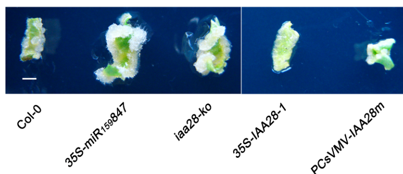
Figure 3. Callus growth in leaf explants (Wang and Guo, 2015). Callus growth in leaf explants of Col-0, 35S-miR159847 transgenic (lines 8), iaa28-ko mutant, and 35S-IAA28-1 and PC5VMV-IAA28m transgenic plants. The explants were photographed on day 7 without changing the medium. Bar = 2 mm.
