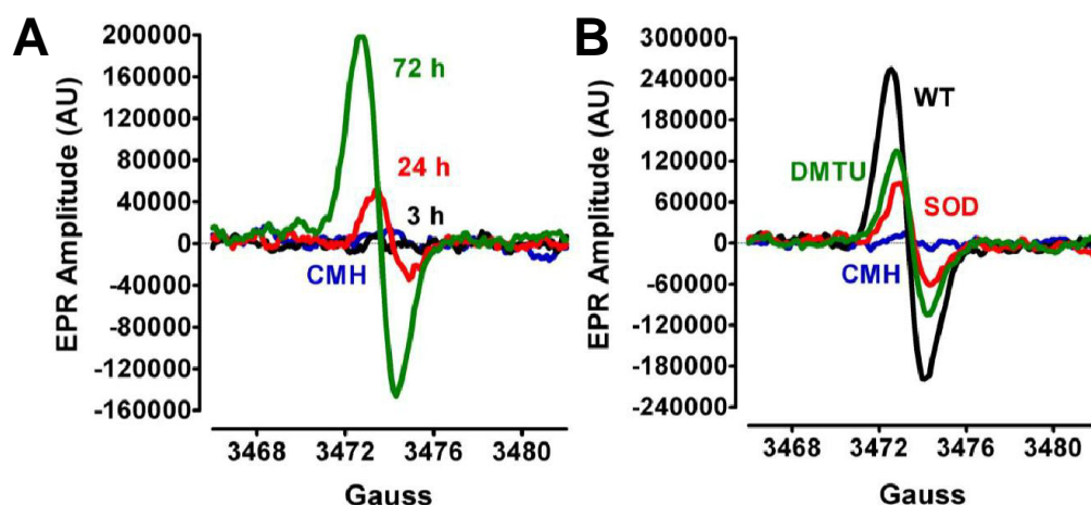
Figure 1. EPR detection of S. aureus ROS production. A. Following inoculation of S. aureus to an initial OD 600 of 0.06, cultures were incubated aerobically (flask: volume ratio= 10:1, 250 rpm). Culture samples for EPR analysis were withdrawn at 3 h, 24 h and 72 h of bacterial growth. B. S. aureus culture samples (72 h) were treated with either 400 units of SOD, 20 mM DMTU, or vehicle (wild-type, WT) before addition of the spin probe, CMH. The basal extent of CMH autoxidation in KDD buffer (blue line) was determined as control.
