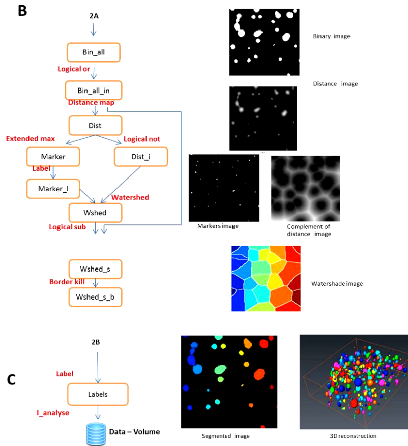
Figure 2. Image analysis pipeline. A. Generating binary images with double thresholding; B. Generating watersheded images; C. Individual labelling of objects and 3 D rendering. The segmentation chain in Avizo (left) and the resulting images (right).
