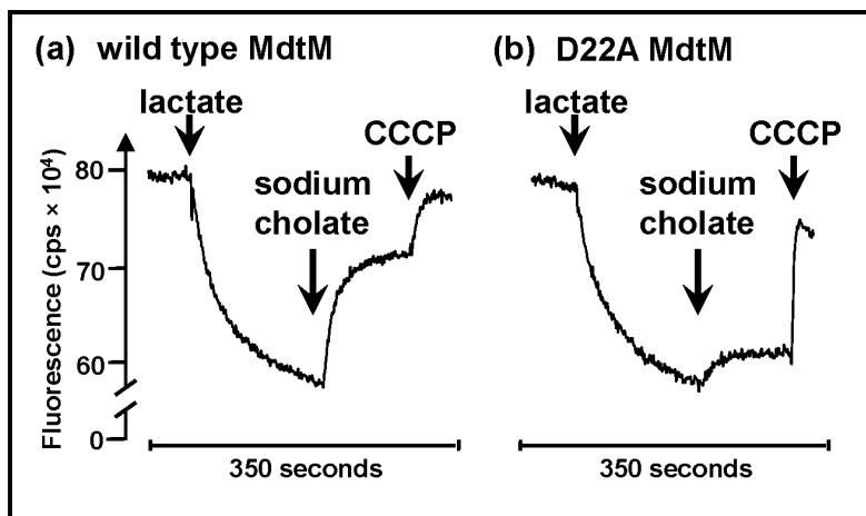
Figure 1. Representative measurements of the fluorescence quench/dequench of acridine orange upon addition of bile salts to inverted vesicles of E. coli TO114 cells that overproduced recombinant (a) wild type MdtM or, as a control, (b) the dysfunctional MdtM D22A mutant. Respiration-dependent generation of \Delta pH (acid inside) was established by addition of sodium DL-lactate as indicated. Sodium cholate was added to vesicles as indicated to initiate the transport reaction and CCCP was used to dissipate \Delta pH. The fluorescence dequench observed in the control experiment (panel b) upon addition of sodium cholate is due to antiport activity of chromosomally encoded MdtM. Fluorescence intensity is measured in counts per second (cps). Note that the fluorescence intensity you measure may differ depending upon how your instrument is set up. The traces above are representative of experiments performed in triplicate on at least two separate preparations of inverted vesicles.
